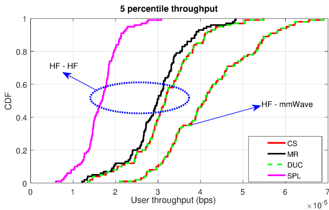
Fig. 4. Comparison of HF-HF versus HF-mmWave network
