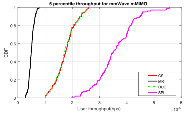
Fig. 3. Throughput with spectral efficiency based user-cell association
