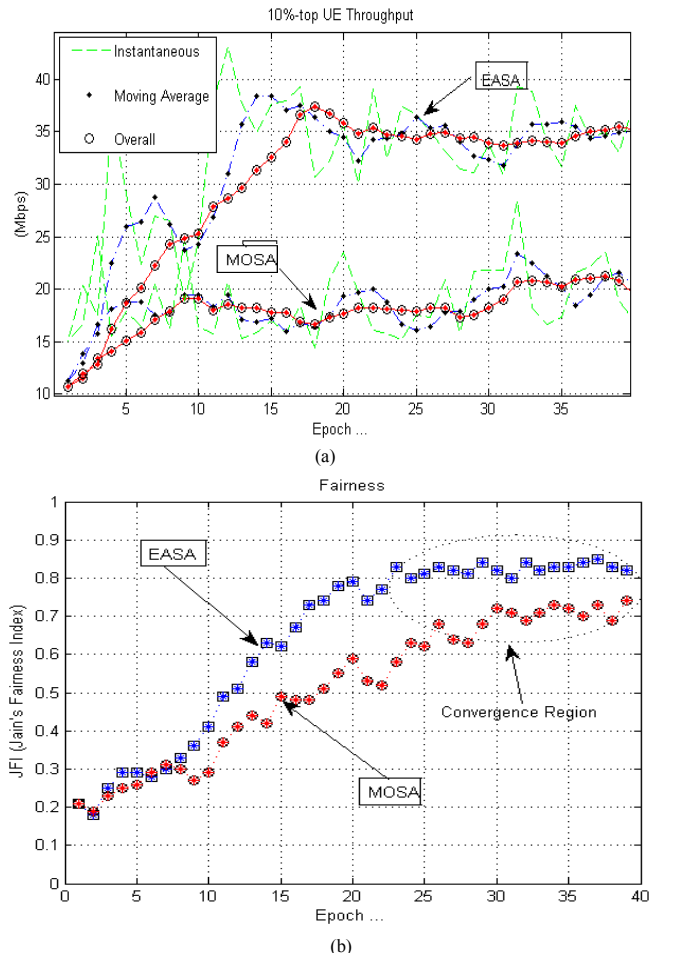
Figure 6: UE Throughput (a) and Jain's Fairness (b) Results in EASA and MOSA
