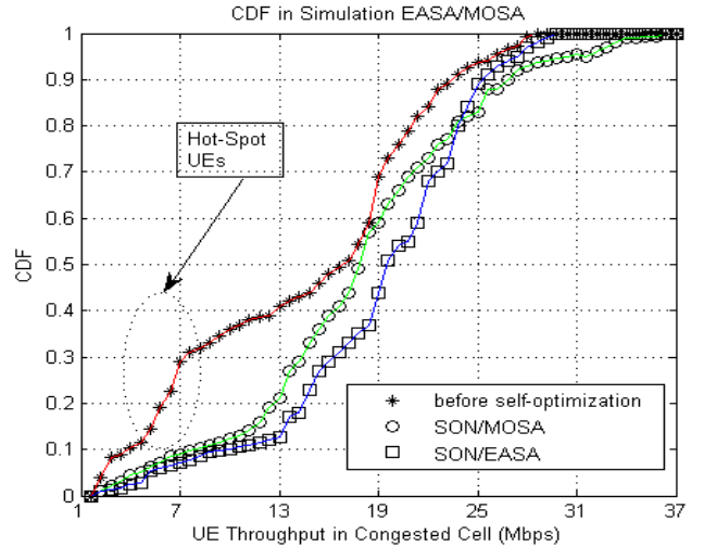
Figure 5: CDF in Simulation: EASA and MOSA Methods
