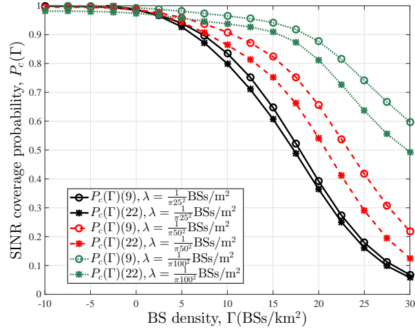
Fig. 12. SINR coverage probability with p(r) being approximated by a step function S_{R_B}(t) in the uplink of mmWave cellular networks.
