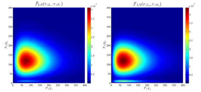
Fig. 5. Joint densities of R_{zL1} and R_{zN2} for the actual PPP model (left) and the independence assumption (right). R_{zL1} and R_{zN2} are the distances of LOS and NLOS users to their respective BSs in two neighboring cells.
