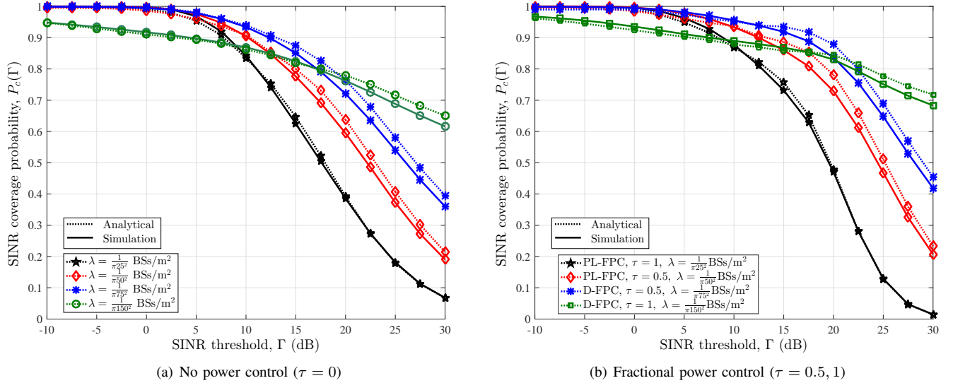
Fig. 6. SINR coverage probability in the uplink channel of mmWave cellular networks
