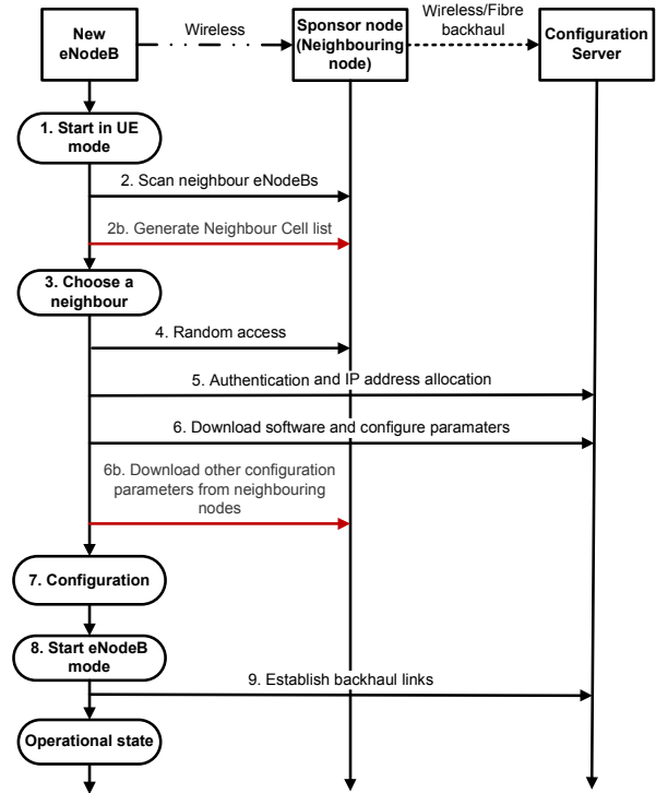
Fig. 4. Self Configuration Flow Chart
