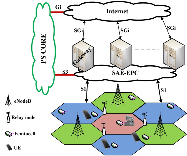
Fig. 3. LTE System Architecture
