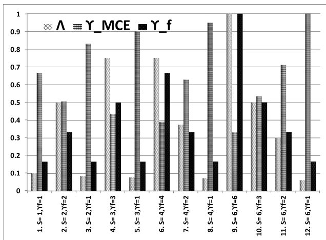
Fig. 2. Quantification of the trade-off between capacity and QoS using proposed metrics. For comparison on same scale, each metric is normalized by its maximum value.
