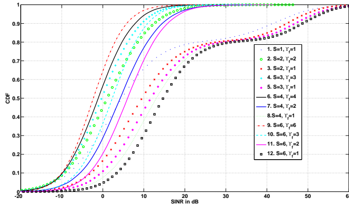
Fig. 1. CDFs of SINR geographical distribution in the coverage area for different number of sectors per site and frequency reuse.
